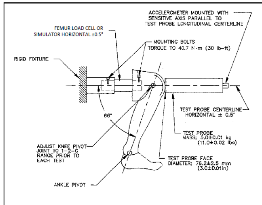
Fig 6: Knee impact test setup specifications
