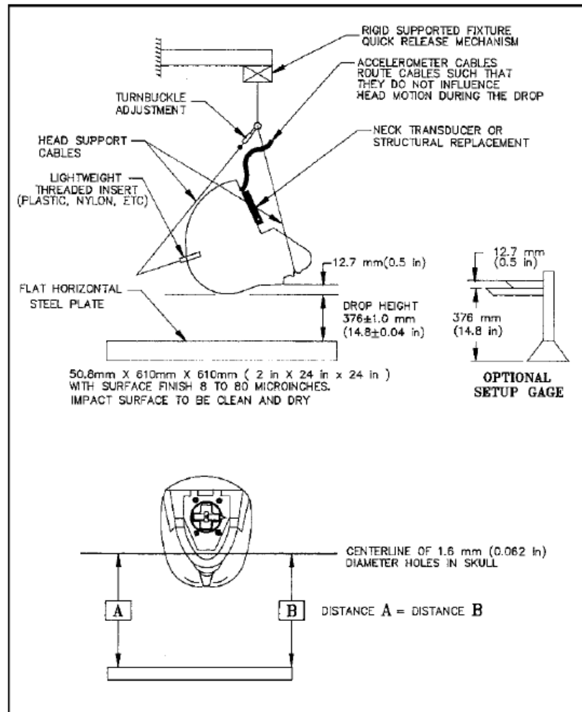
Fig 2: Head drop test setup.
