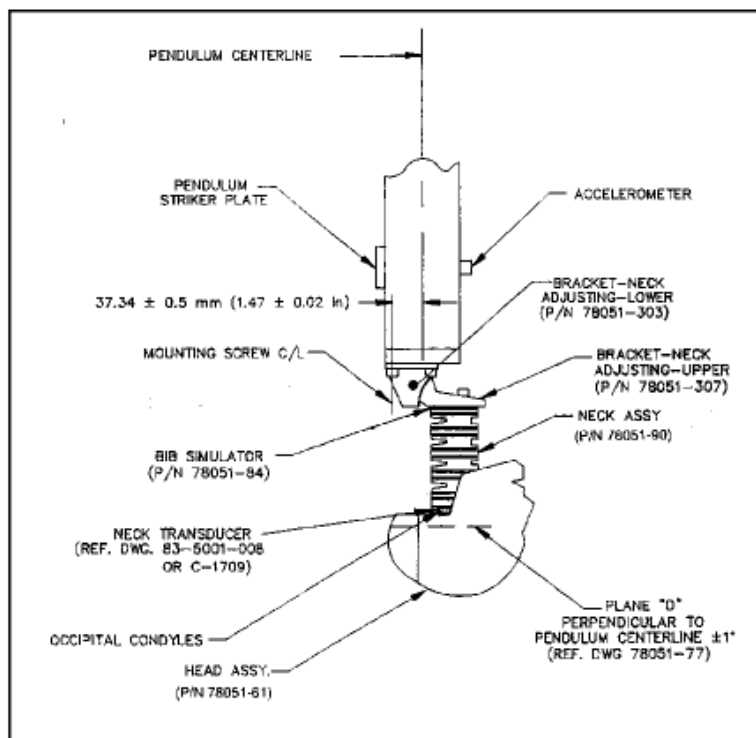
Fig 5: Neck flexion test setup.
