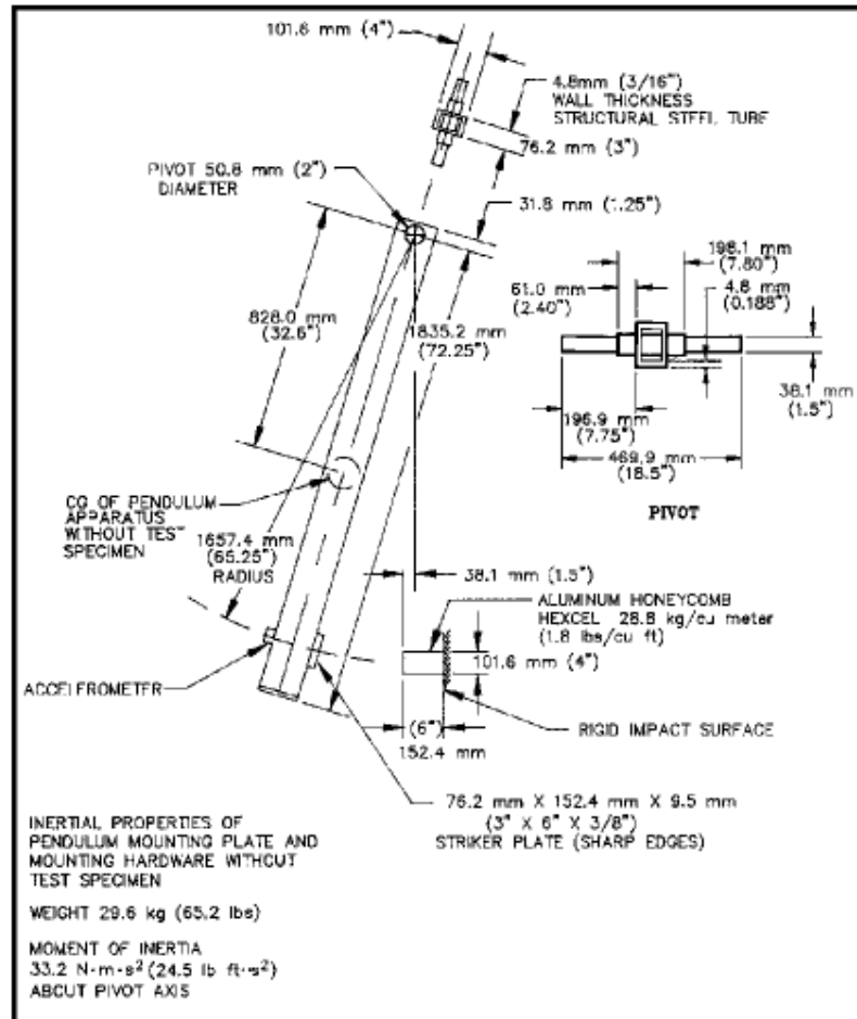
Fig 3: Neck pendulum arm specifications.
