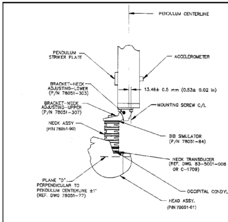
Fig 4: Neck flexion test setup.
