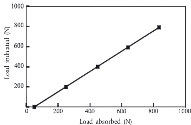
Figure 2 Load indicated at 80 km/h in terms of load absorbed at 80 km/h
