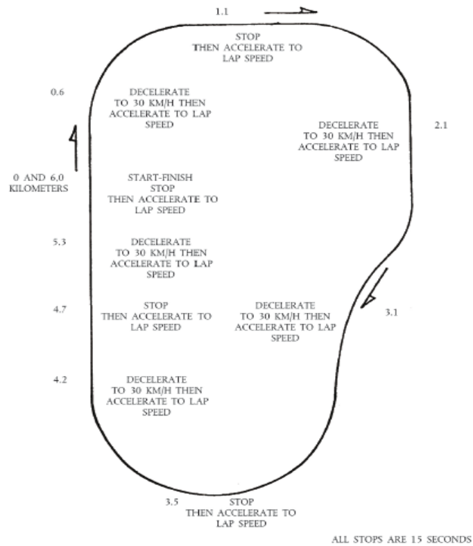
Figure 1 Driving schedule AMA test sub-sub-cycle
