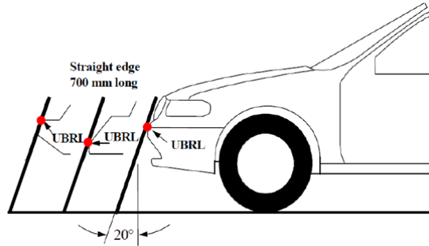
Figure 9 Upper Bumper Reference Line (UBRL)
