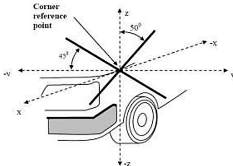
Figure 26: Corner reference point (as referred in clause 3.32)
