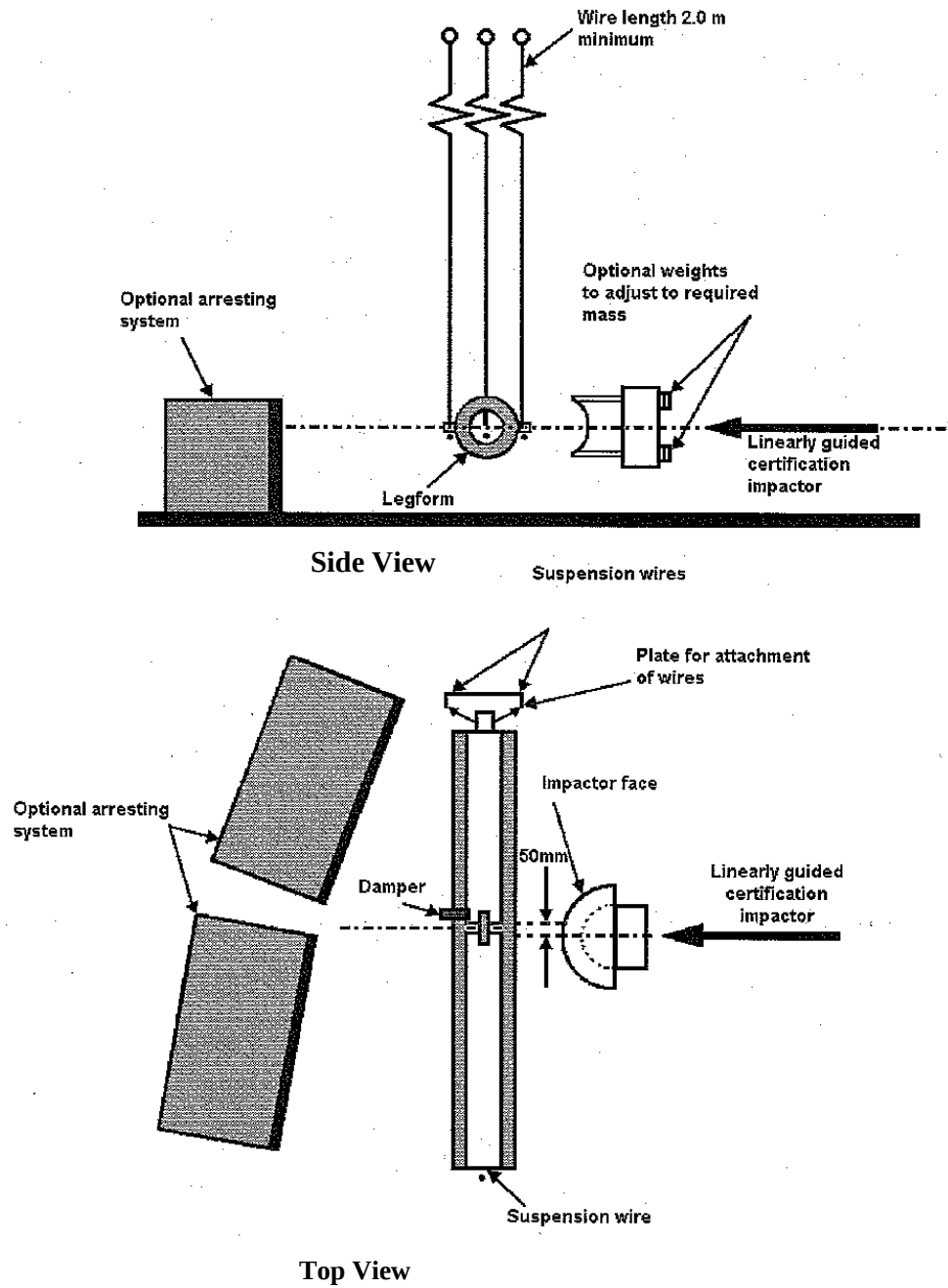
Figure 22 Test Set up for Dynamic Lower Legform Impactor Certification Test
