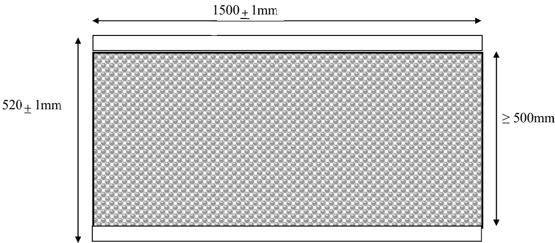
Figure 5 Front View
