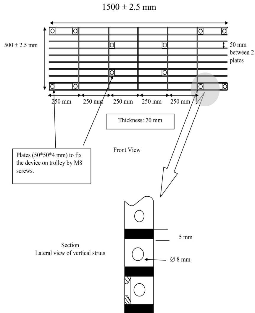
Figure 9 Side View
