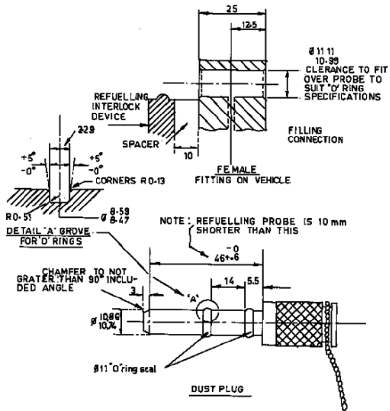
DUST PLUG CNG VEHICLE FILLING SYSTEM
