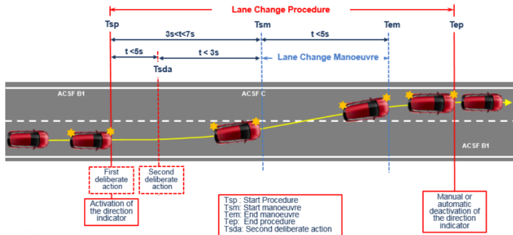
ACSF C – Case where the lateral movement is initiated by a second deliberate action by the driver (2 Step HMI)
