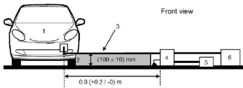
Figure 1c – Front View
