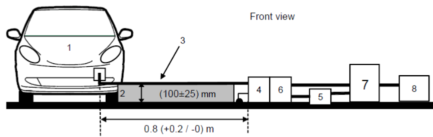
Figure 1c – Front View
