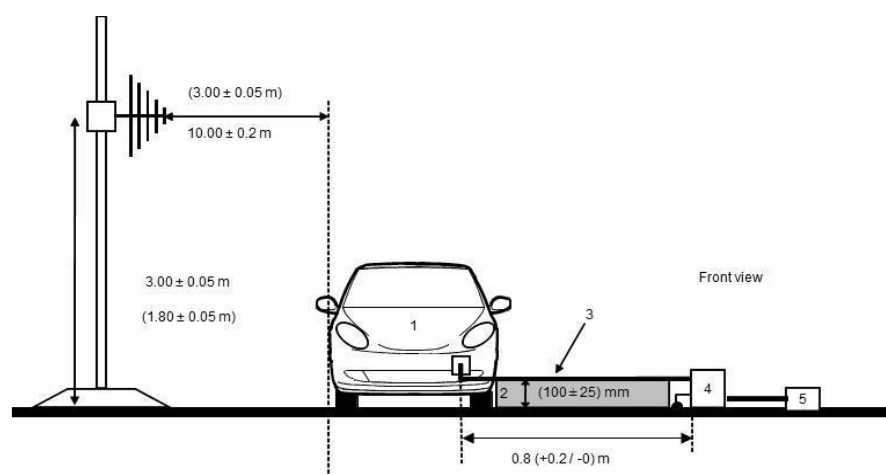
Figure 3c – Front View
