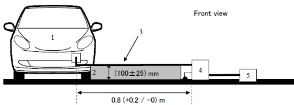
Figure 4c – Front View
