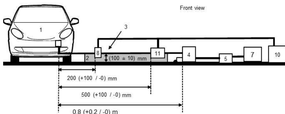
Figure 2c – Front View
